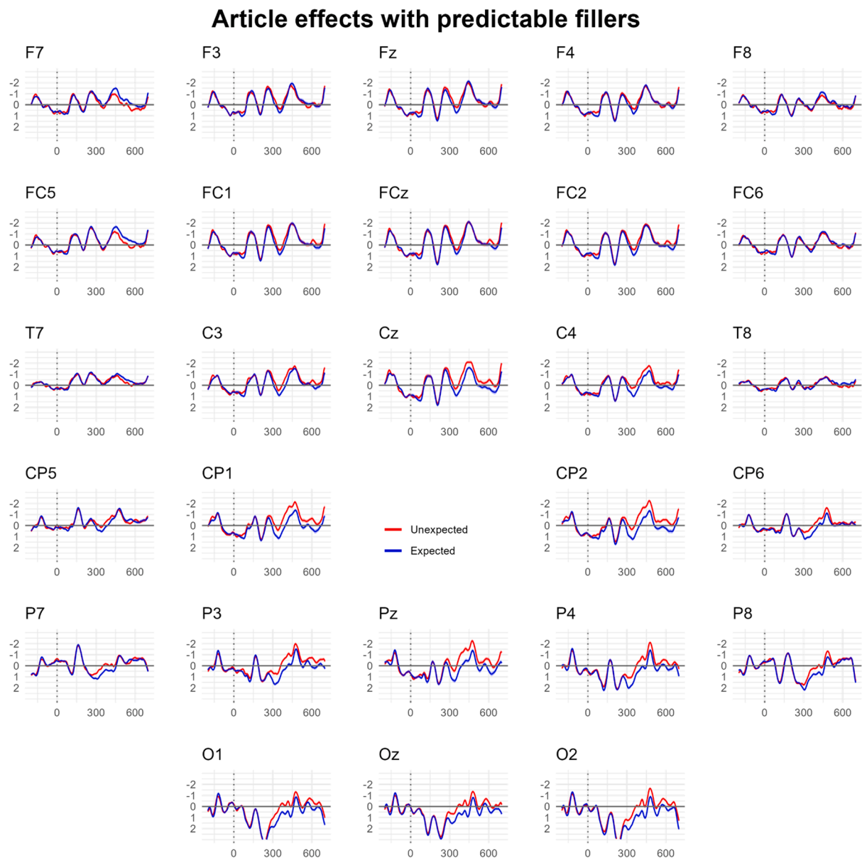
Fig. A1. Article effects with predictable fillers. The graphs show the grand-average ERPs of expected and unexpected articles for each recorded channel.
