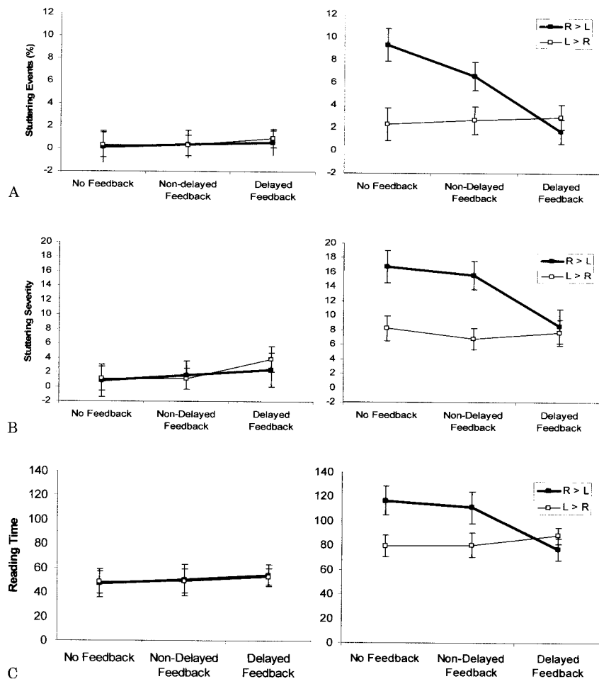
Figure 2. Structure–function relationships in developmental stuttering. Relationships and means associated with the significant Group \times delayed auditory feedback (DAF) condition \times planum temporale (PT) asymmetry interactions are shown for each fluency measure. The frequency of stuttering events variable is depicted in A, the stuttering severity variable is depicted in B, and the reading time variable is depicted in C. Error bars represent standard error (SE) of the mean.
